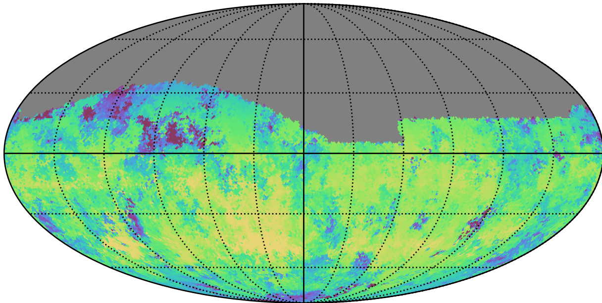
ddf_loaded_fl2_v3.4_10yrs Yr 1 i band: Median skyBrightness
