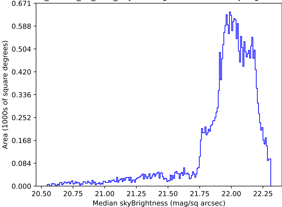
ddf_loaded_fl2_v3.4_10yrs Yr 1 g band: Median skyBrightness
