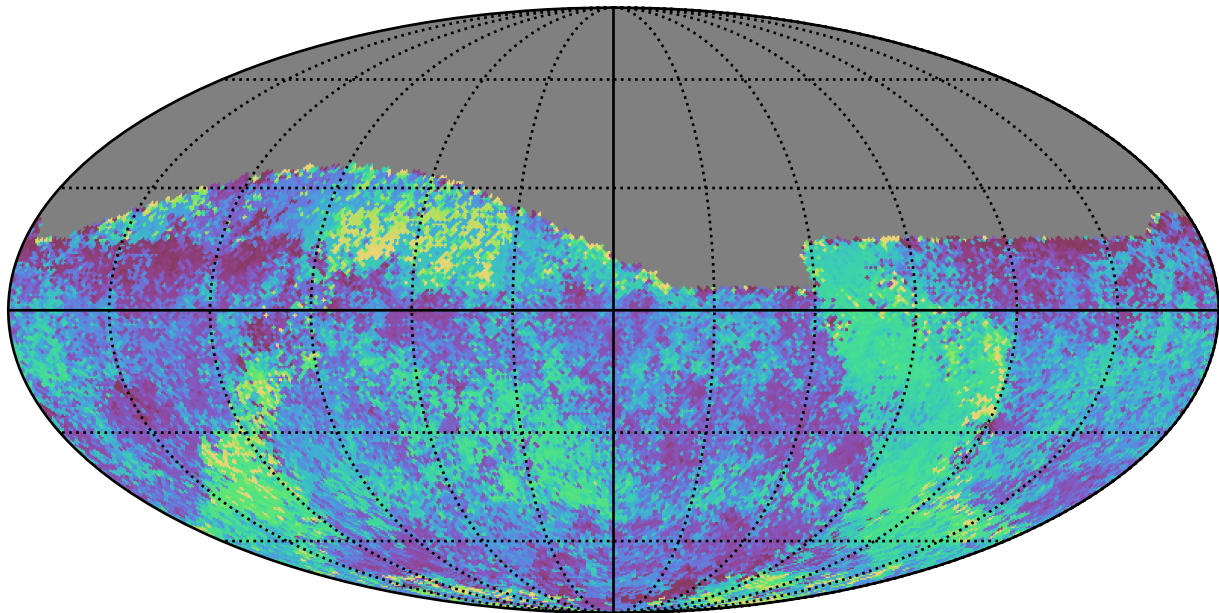
ddf_loaded_fl2_v3.4_10yrs Yr 1 all bands: Median skyBrightness
