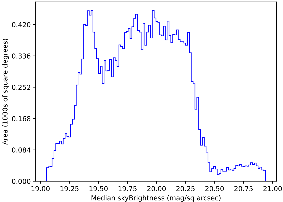
ddf_loaded_fl2_v3.4_10yrs Yr 1 all bands: Median skyBrightness
