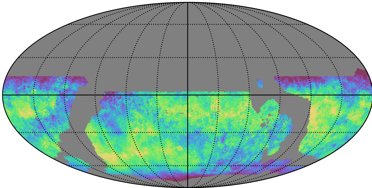
ddf_loaded_fl2_v3.4_10yrs WFD z band: Median skyBrightness
