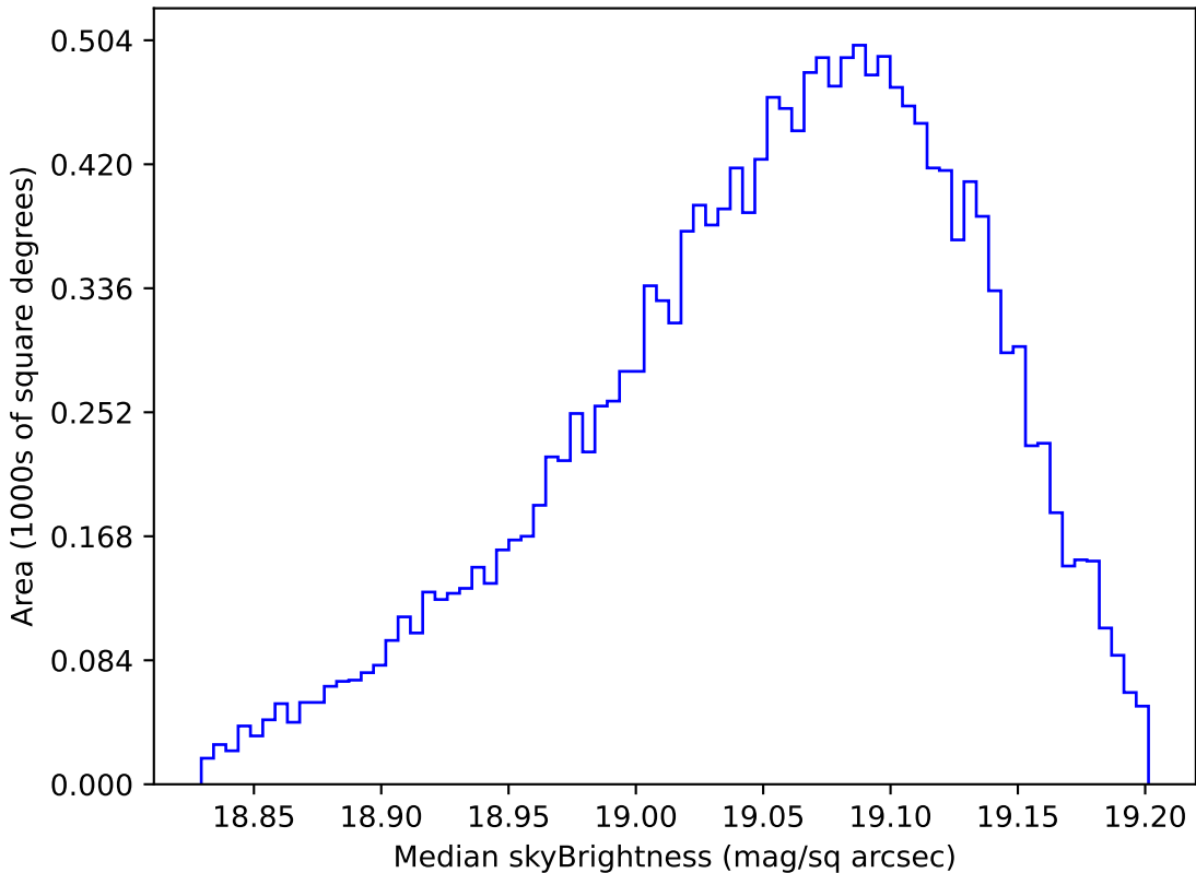
ddf_loaded_fl2_v3.4_10yrs WFD z band: Median skyBrightness
