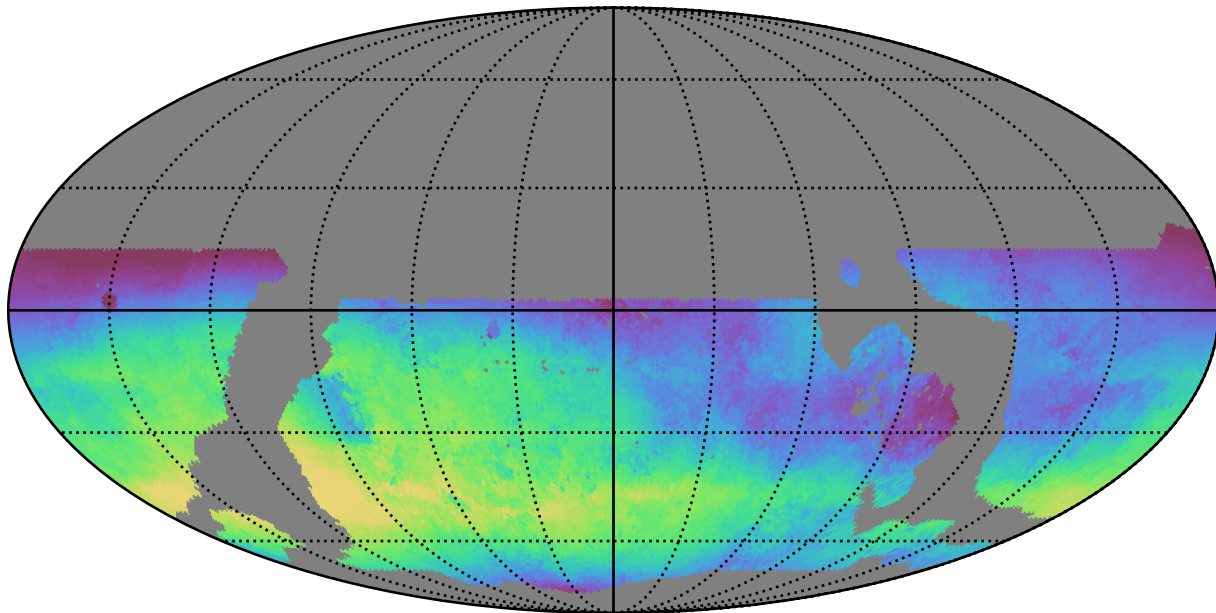
ddf_loaded_fl2_v3.4_10yrs WFD u band: Median skyBrightness
