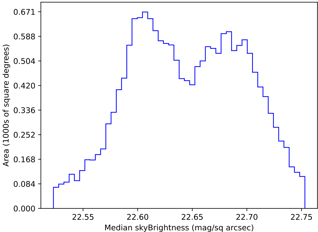
ddf_loaded_fl2_v3.4_10yrs WFD u band: Median skyBrightness
