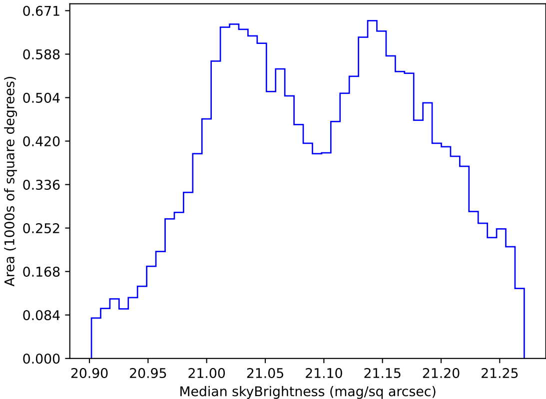
ddf_loaded_fl2_v3.4_10yrs WFD r band: Median skyBrightness
