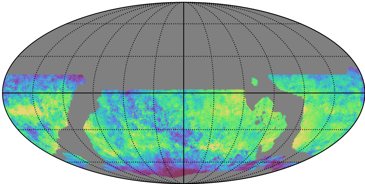
ddf_loaded_fl2_v3.4_10yrs WFD i band: Median skyBrightness
