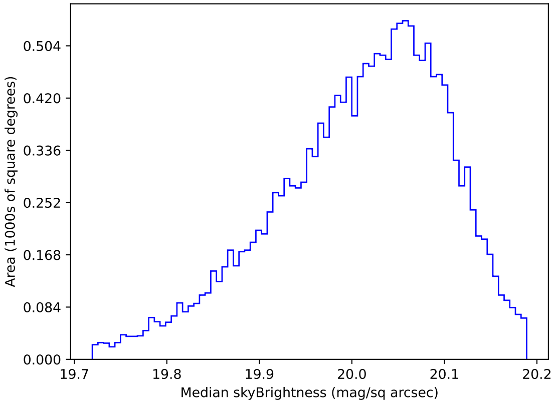
ddf_loaded_fl2_v3.4_10yrs WFD i band: Median skyBrightness
