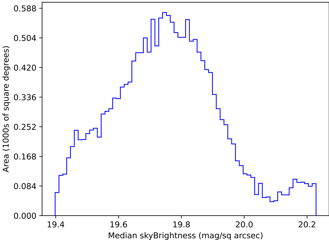
ddf_loaded_fl2_v3.4_10yrs WFD all bands: Median skyBrightness
