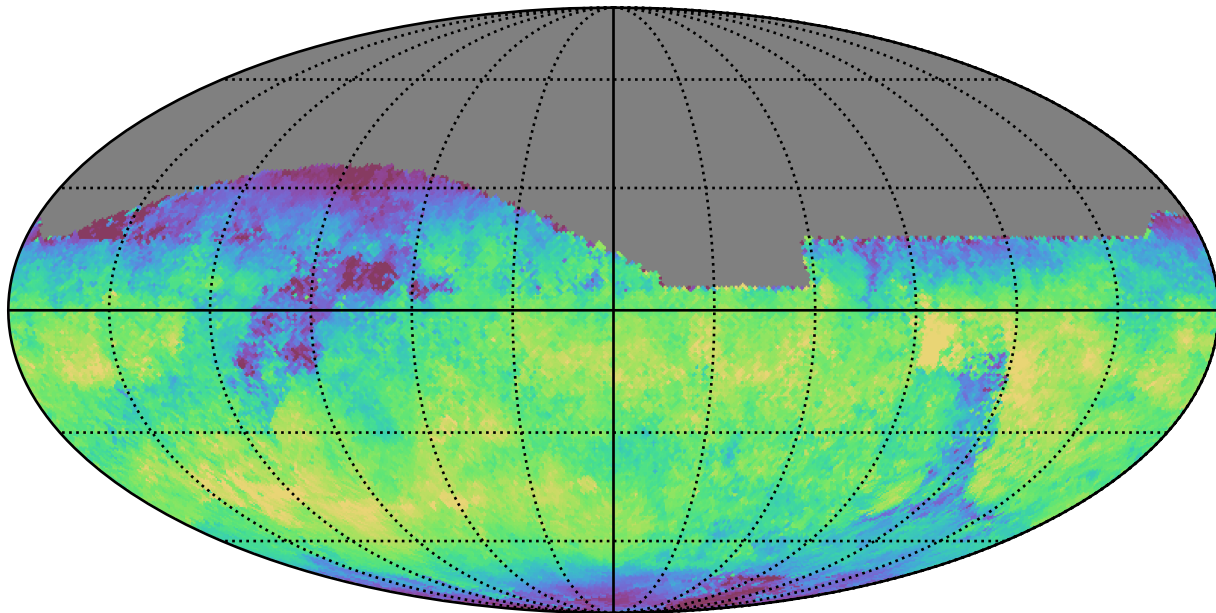
ddf_loaded_fl2_v3.4_10yrs All sky z band: Median skyBrightness
