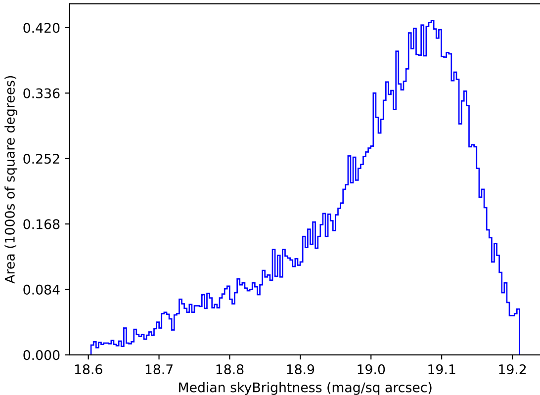
ddf_loaded_fl2_v3.4_10yrs All sky z band: Median skyBrightness
