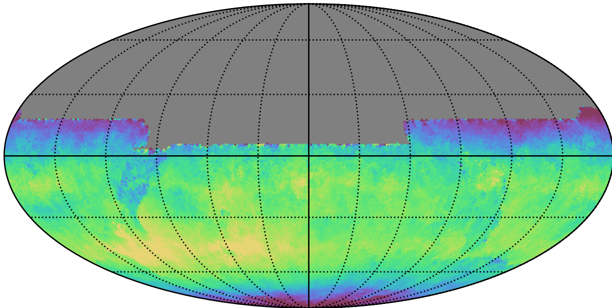
ddf_loaded_fl2_v3.4_10yrs All sky y band: Median skyBrightness
