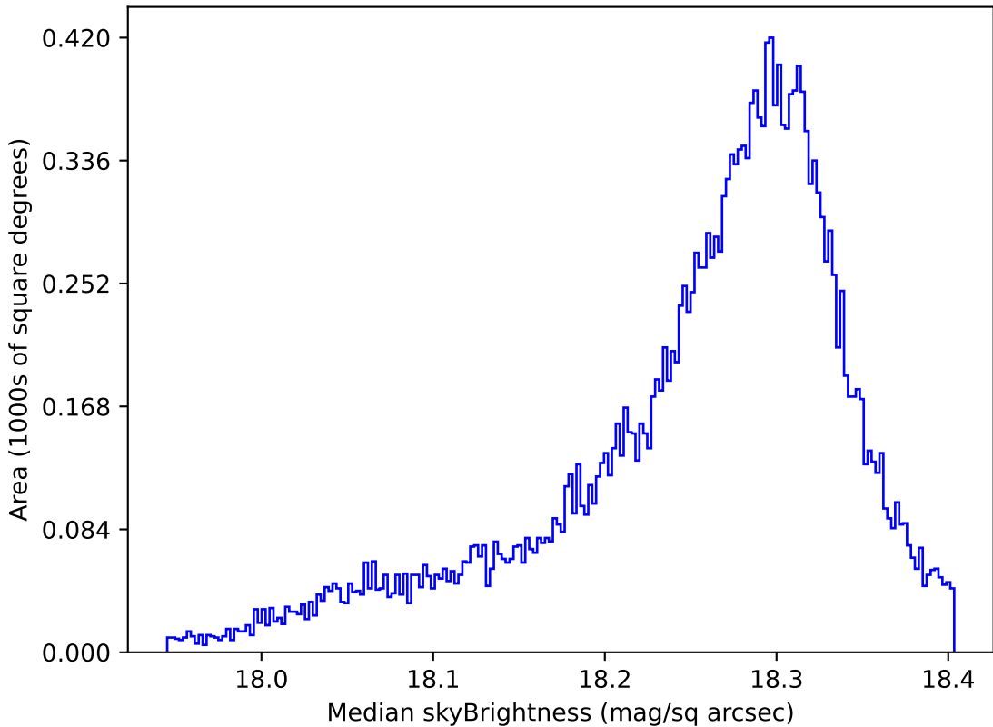
ddf_loaded_fl2_v3.4_10yrs All sky y band: Median skyBrightness
