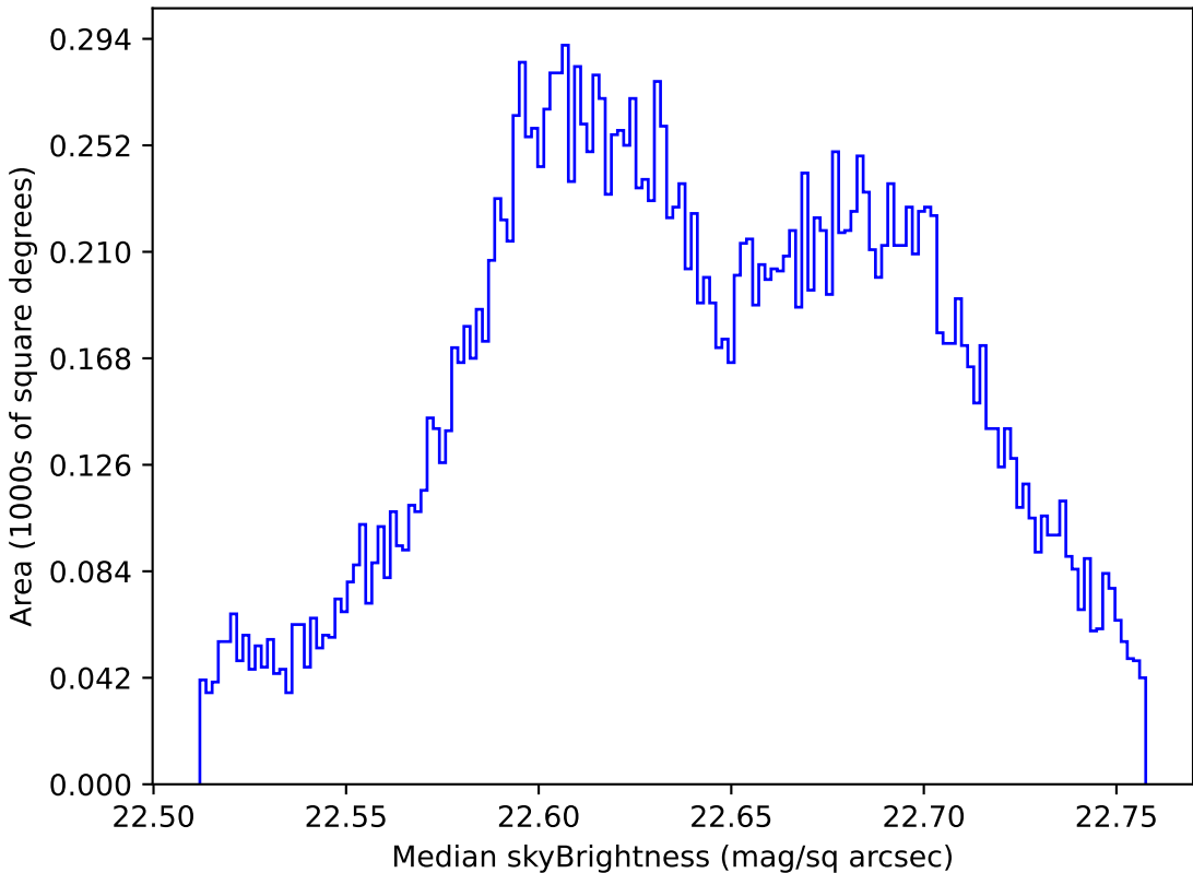
ddf_loaded_fl2_v3.4_10yrs All sky u band: Median skyBrightness
