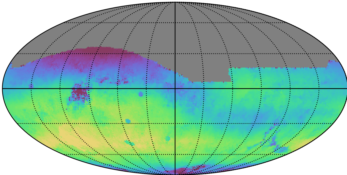
ddf_loaded_fl2_v3.4_10yrs All sky r band: Median skyBrightness
