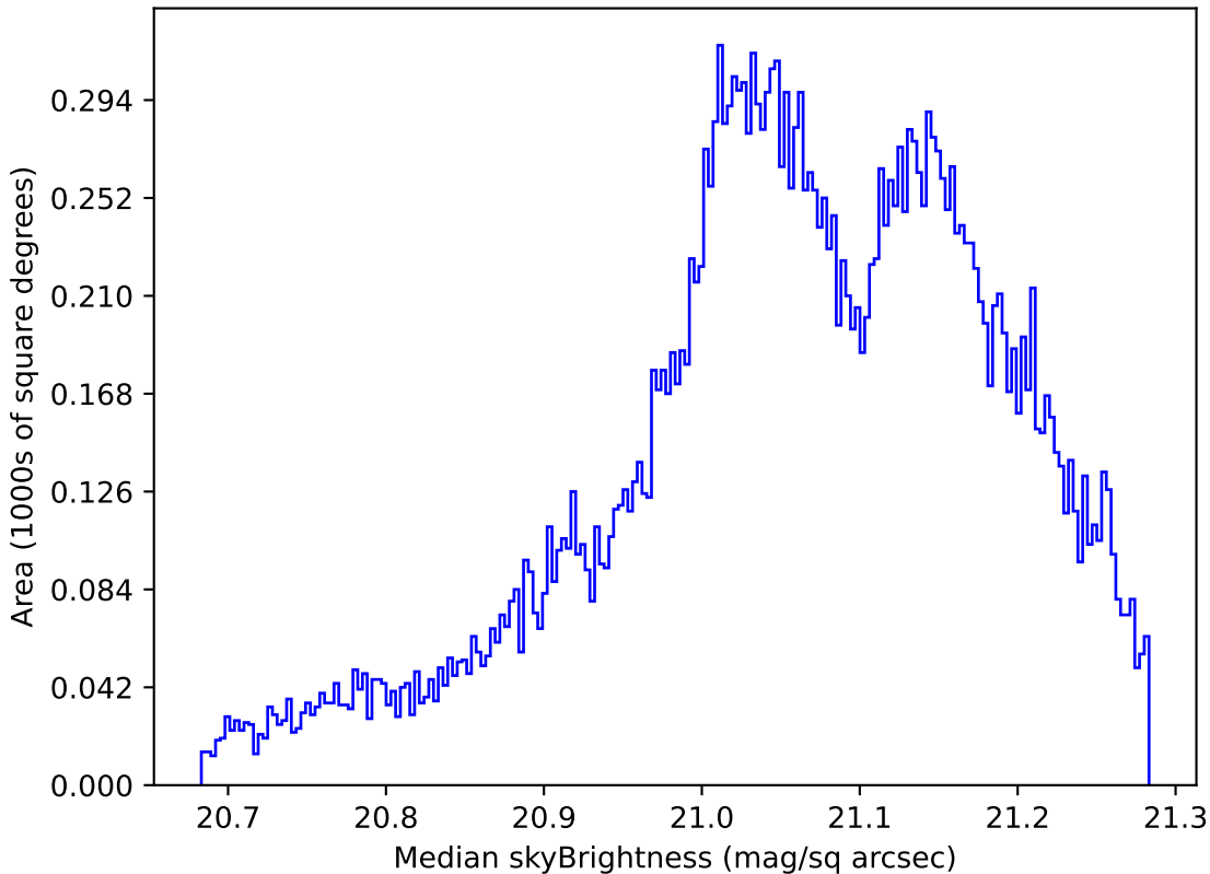
ddf_loaded_fl2_v3.4_10yrs All sky r band: Median skyBrightness
