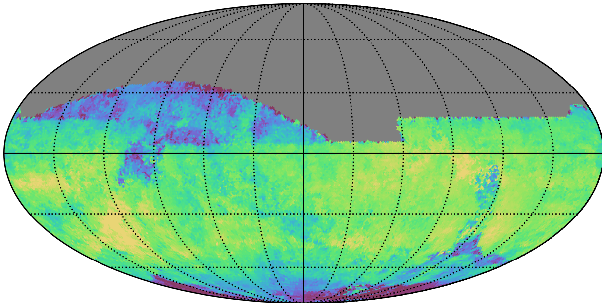
ddf_loaded_fl2_v3.4_10yrs All sky i band: Median skyBrightness
