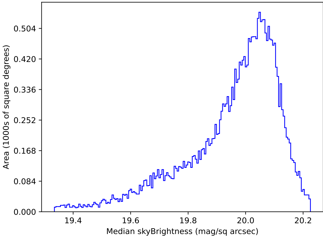
ddf_loaded_fl2_v3.4_10yrs All sky i band: Median skyBrightness
