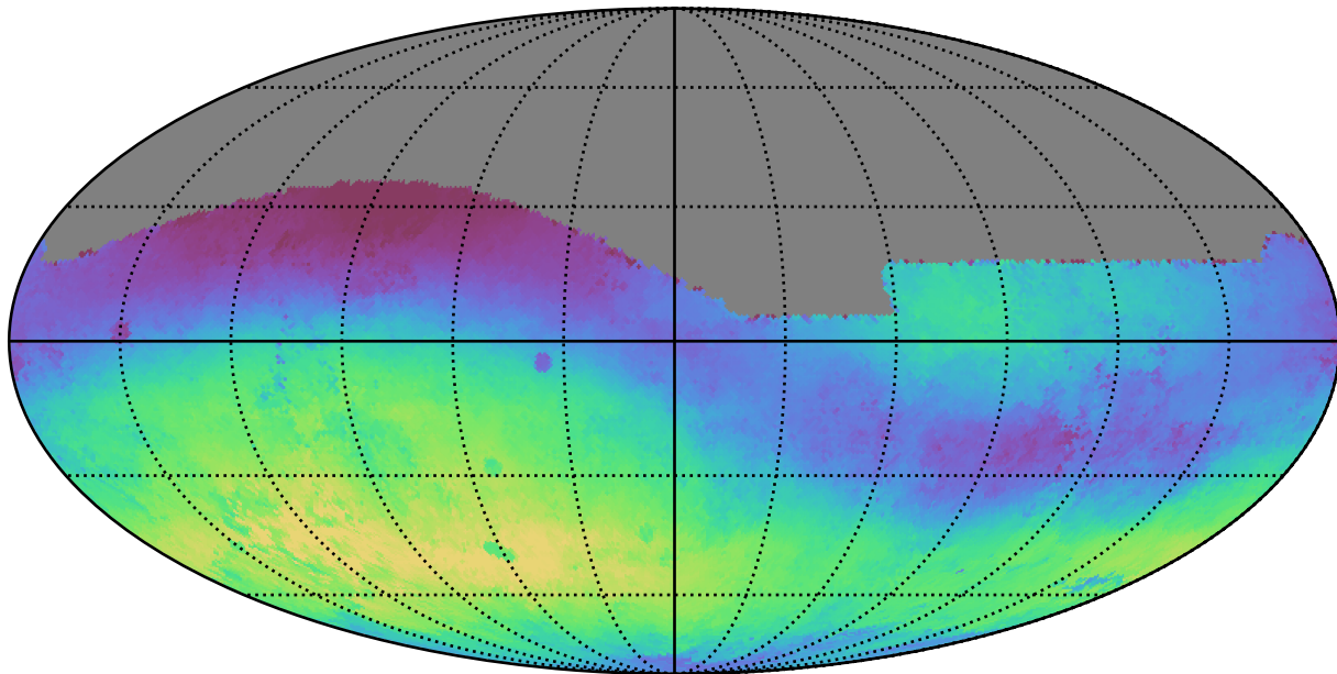
ddf_loaded_fl2_v3.4_10yrs All sky g band: Median skyBrightness
