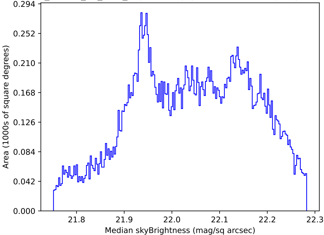
ddf_loaded_fl2_v3.4_10yrs All sky g band: Median skyBrightness
