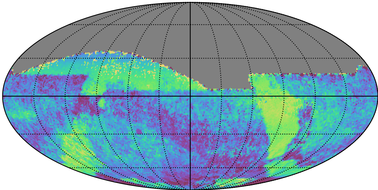
ddf_loaded_fl2_v3.4_10yrs All sky all bands: Median skyBrightness
