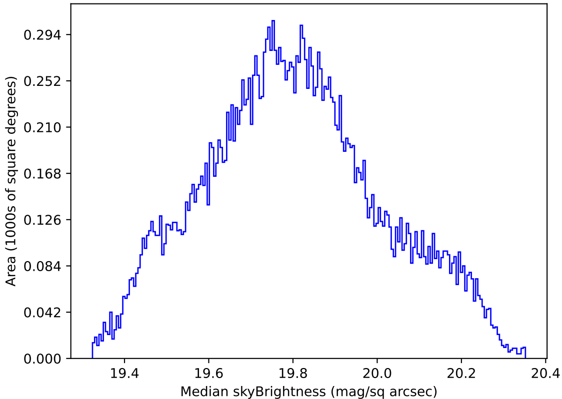
ddf_loaded_fl2_v3.4_10yrs All sky all bands: Median skyBrightness
