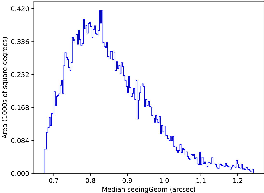
ddf_loaded_fl2_v3.4_10yrs Yr 1 z band: Median seeingGeom
