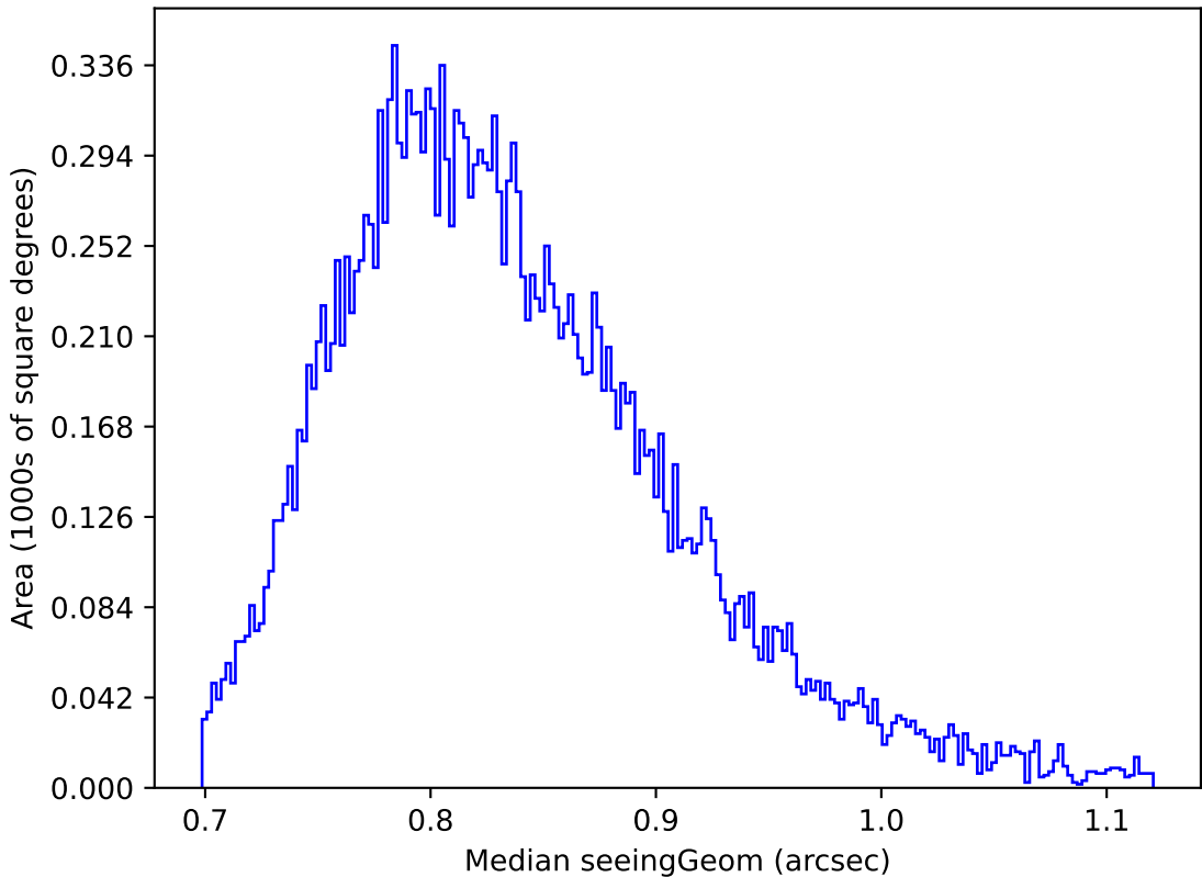
ddf_loaded_fl2_v3.4_10yrs Yr 1 y band: Median seeingGeom
