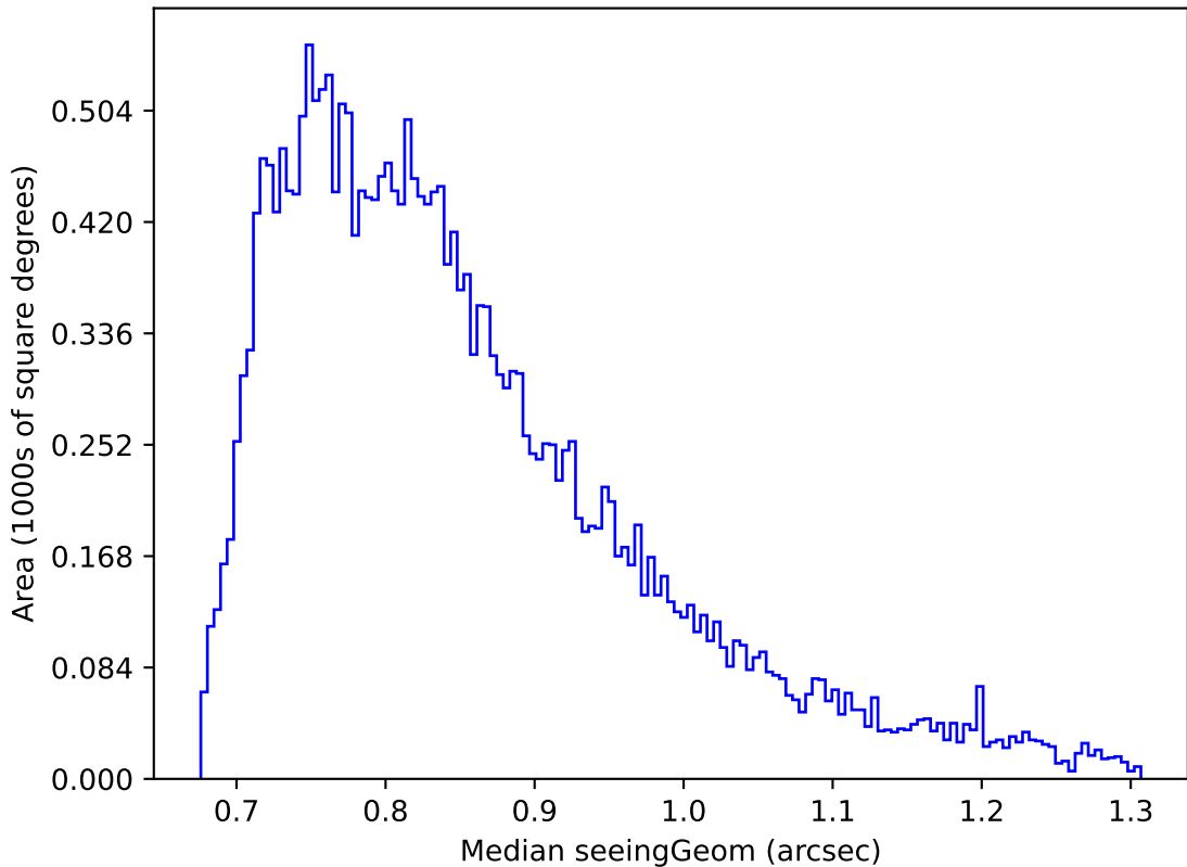
ddf_loaded_fl2_v3.4_10yrs Yr 1 r band: Median seeingGeom
