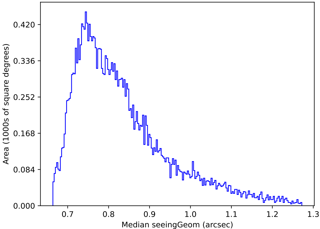
ddf_loaded_fl2_v3.4_10yrs Yr 1 i band: Median seeingGeom
