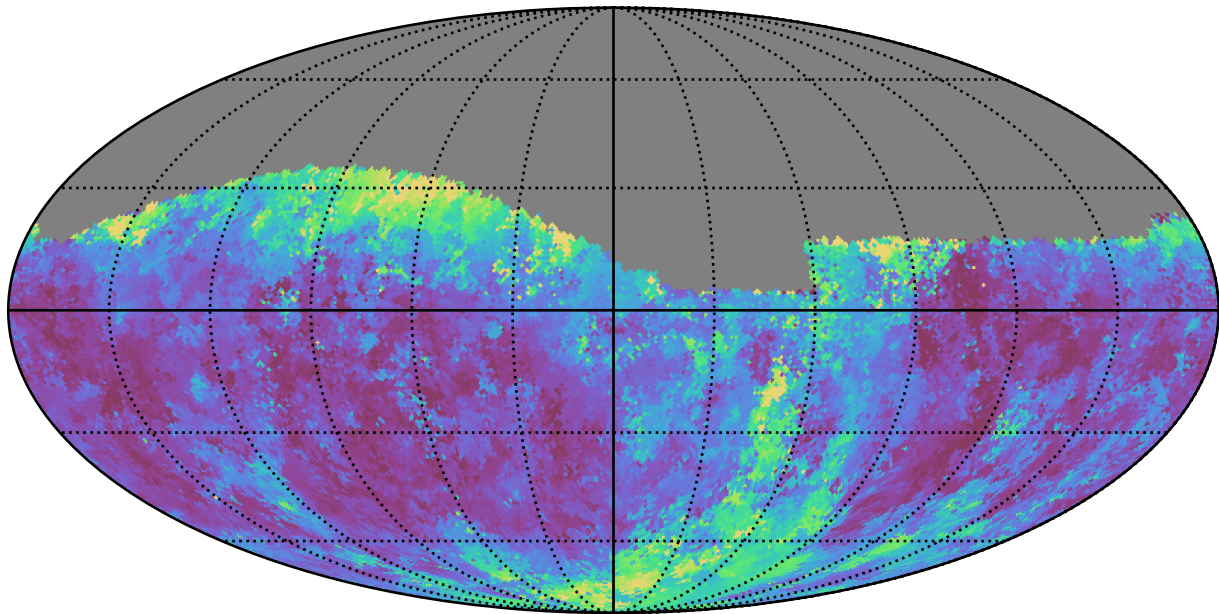
ddf_loaded_fl2_v3.4_10yrs Yr 1 g band: Median seeingGeom
