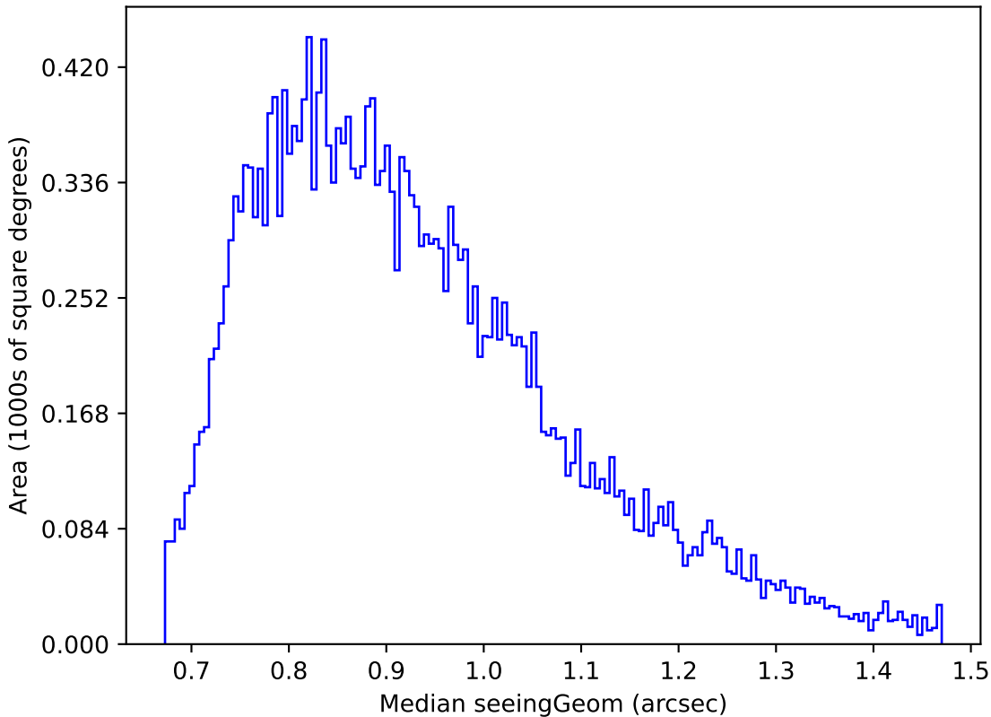
ddf_loaded_fl2_v3.4_10yrs Yr 1 g band: Median seeingGeom
