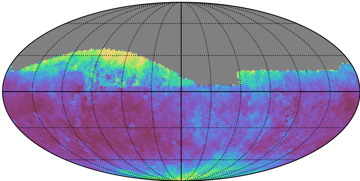
ddf_loaded_fl2_v3.4_10yrs Yr 1 all bands: Median seeingGeom
