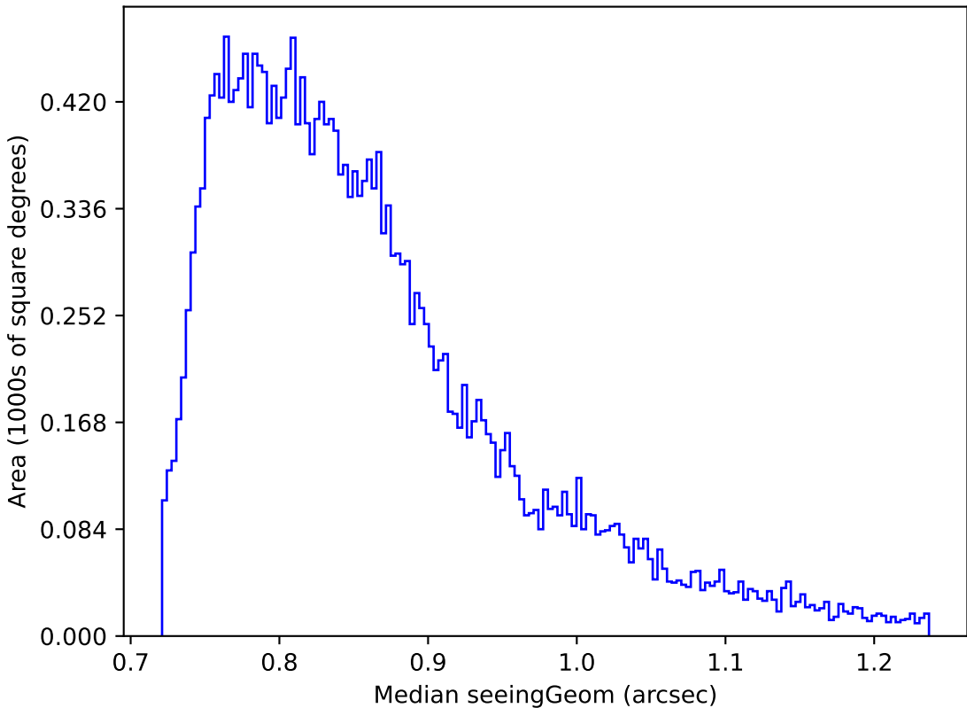
ddf_loaded_fl2_v3.4_10yrs Yr 1 all bands: Median seeingGeom
