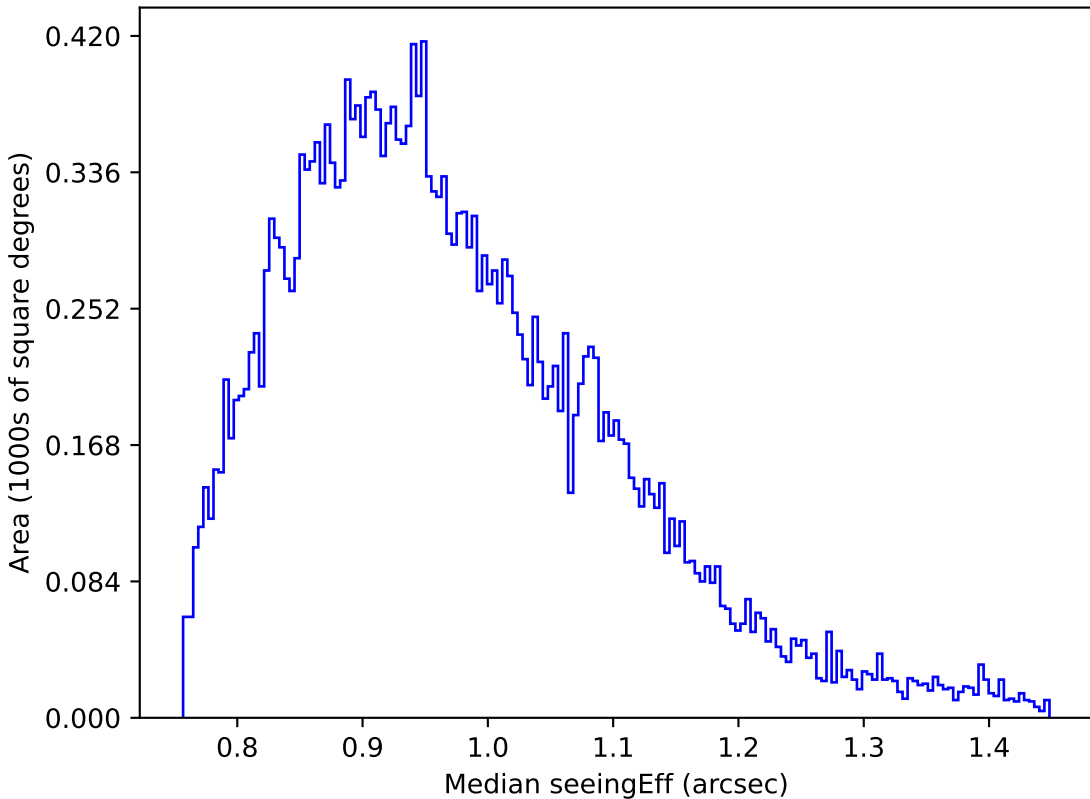
ddf_loaded_fl2_v3.4_10yrs Yr 1 z band: Median seeingEff
