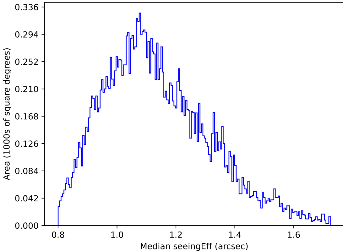
ddf_loaded_fl2_v3.4_10yrs Yr 1 u band: Median seeingEff
