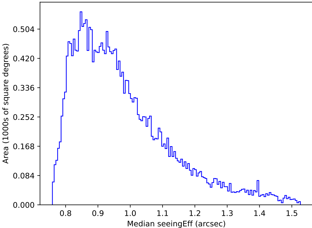
ddf_loaded_fl2_v3.4_10yrs Yr 1 r band: Median seeingEff
