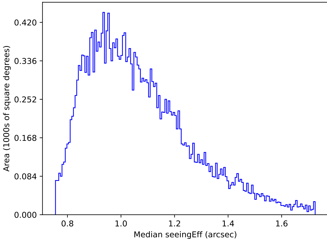
ddf_loaded_fl2_v3.4_10yrs Yr 1 g band: Median seeingEff
