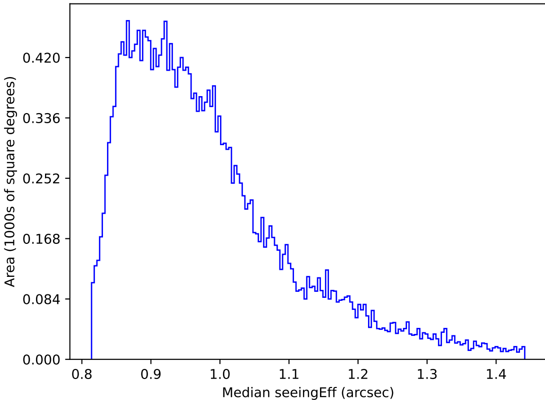
ddf_loaded_fl2_v3.4_10yrs Yr 1 all bands: Median seeingEff
