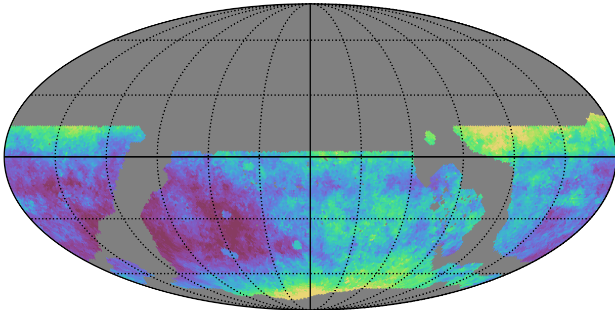
ddf_loaded_fl2_v3.4_10yrs WFD z band: Median seeingEff
