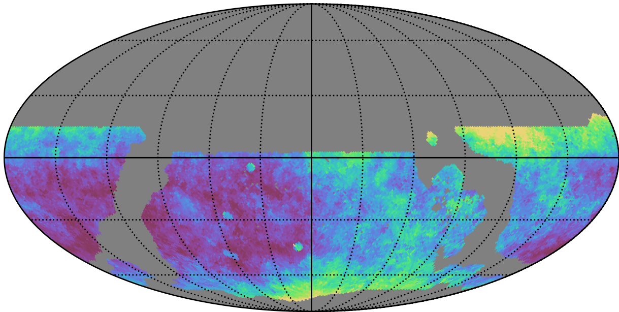
ddf_loaded_fl2_v3.4_10yrs WFD y band: Median seeingEff
