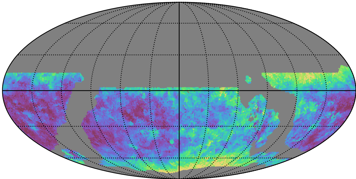
ddf_loaded_fl2_v3.4_10yrs WFD u band: Median seeingEff
