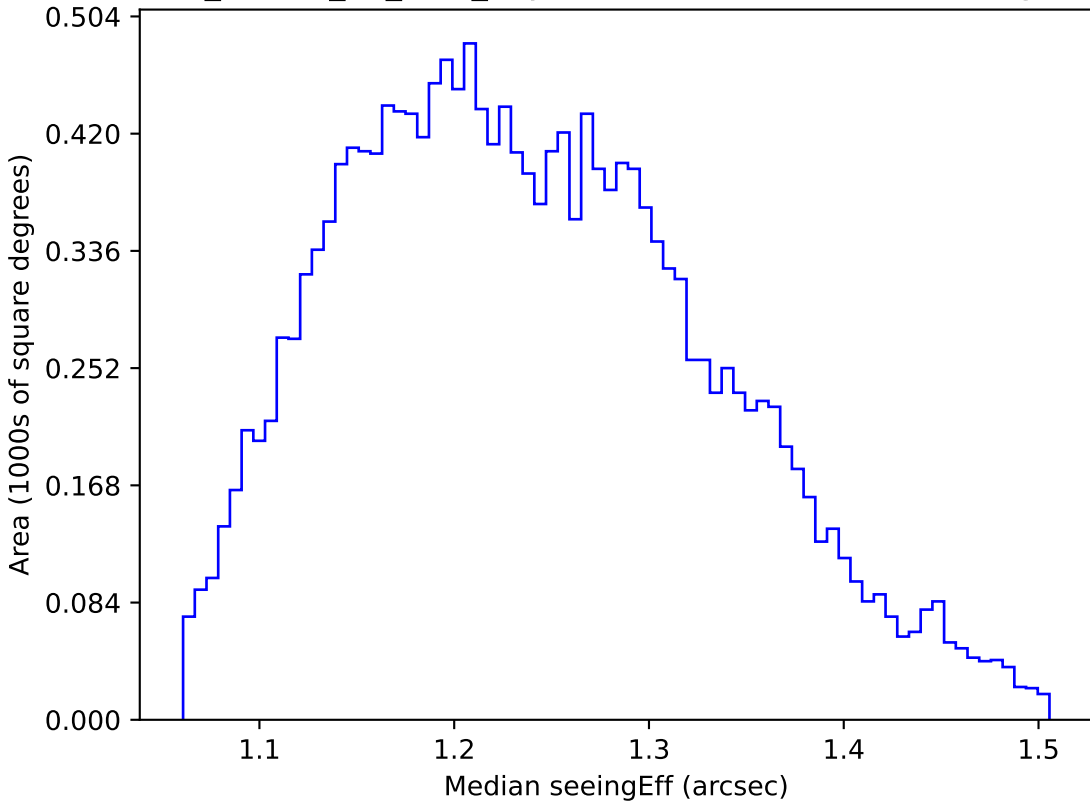
ddf_loaded_fl2_v3.4_10yrs WFD u band: Median seeingEff
