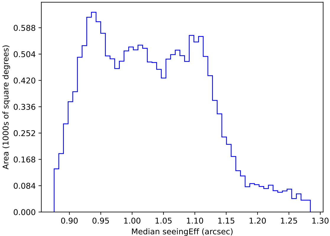
ddf_loaded_fl2_v3.4_10yrs WFD r band: Median seeingEff
