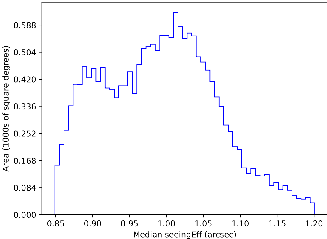
ddf_loaded_fl2_v3.4_10yrs WFD i band: Median seeingEff
