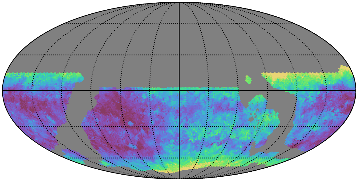
ddf_loaded_fl2_v3.4_10yrs WFD g band: Median seeingEff
