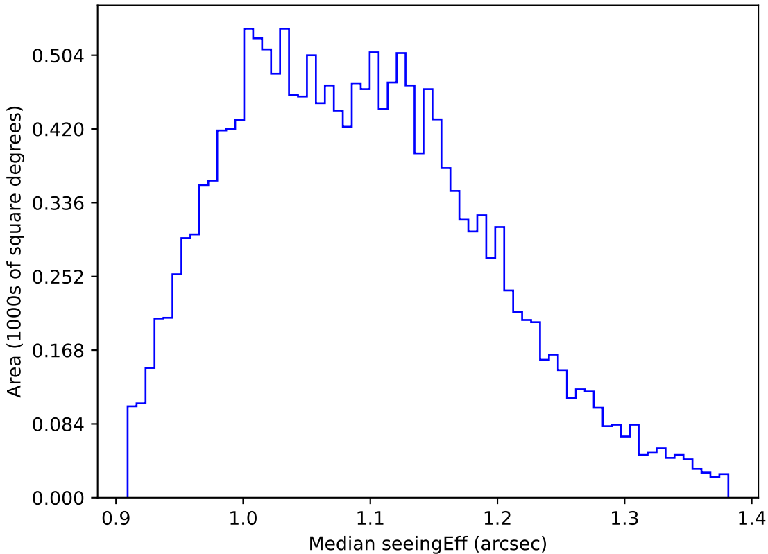
ddf_loaded_fl2_v3.4_10yrs WFD g band: Median seeingEff
