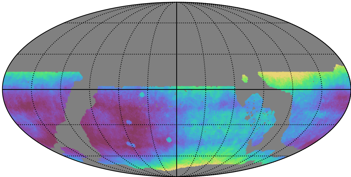
ddf_loaded_fl2_v3.4_10yrs WFD all bands: Median seeingEff
