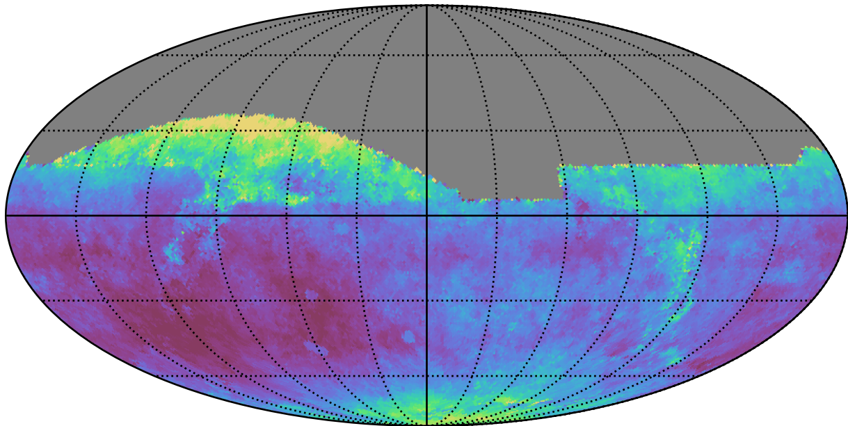
ddf_loaded_fl2_v3.4_10yrs All sky z band: Median seeingEff
