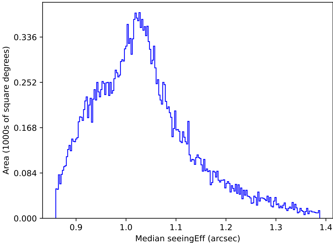
ddf_loaded_fl2_v3.4_10yrs All sky z band: Median seeingEff
