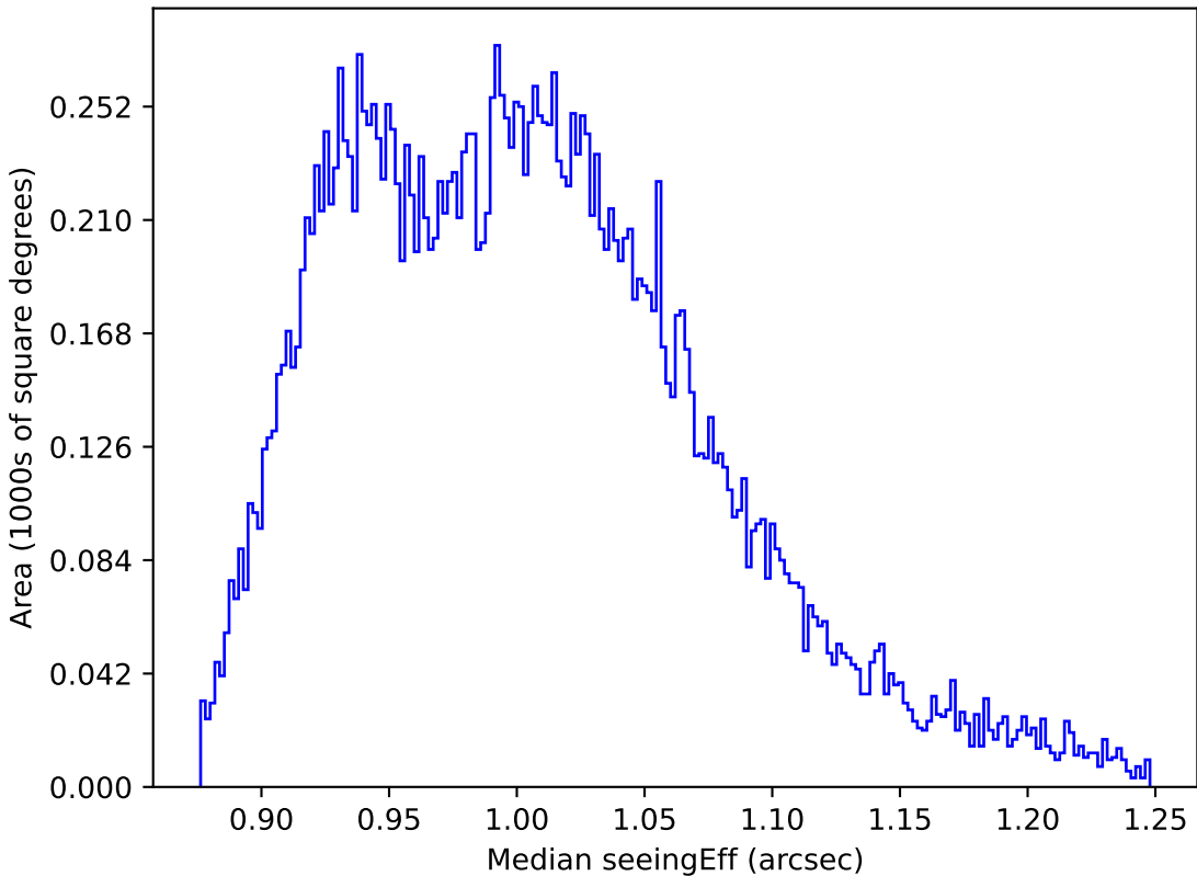
ddf_loaded_fl2_v3.4_10yrs All sky y band: Median seeingEff
